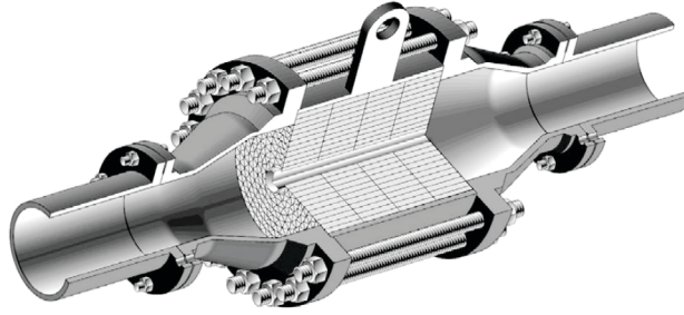
Figure 2. Cut-away view of EN-DFA Series Detonation Flame Arrestor
