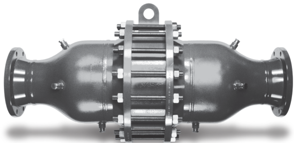
Figure 1. Typical EN-DFA Series Detonation Flame Arrestor
