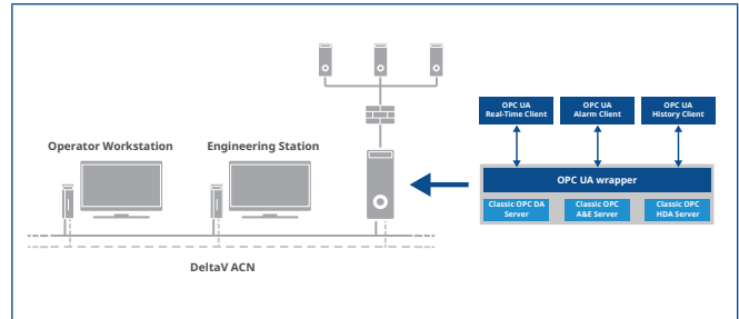
DeltaV OPC UA server in the Application Station providing a single point of connection for DA, HDA and A&E.
