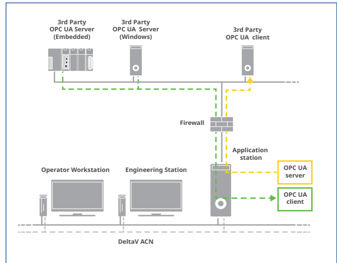
Application station with OPC UA server and client enabled at the same time and connected with 3rd party OPC UA servers and clients.
