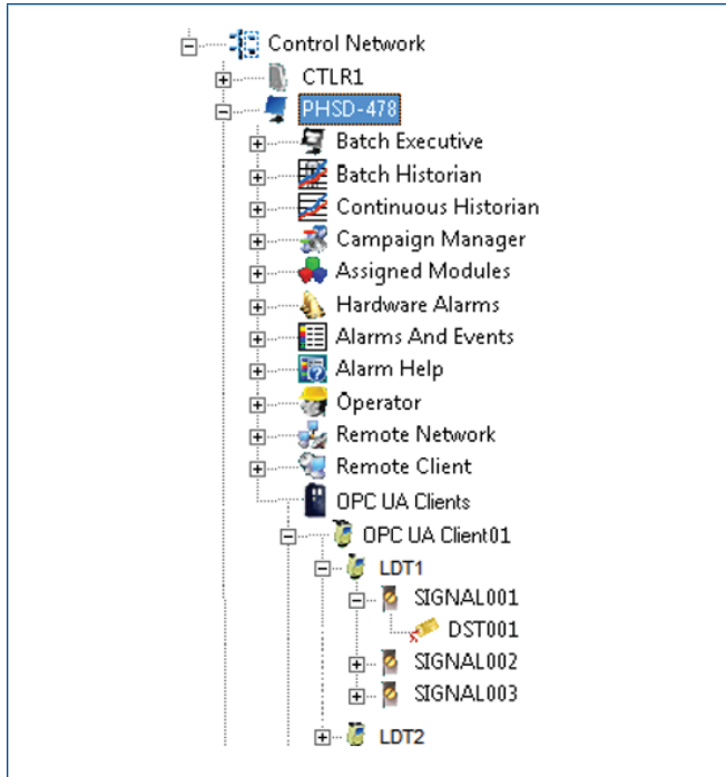
DeltaV Explorer showing the DeltaV OPC UA client hierarchy in the Application station.
