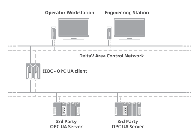
Ethernet I/O card with OPC UA client connected with 3rd party OPC UA servers.
