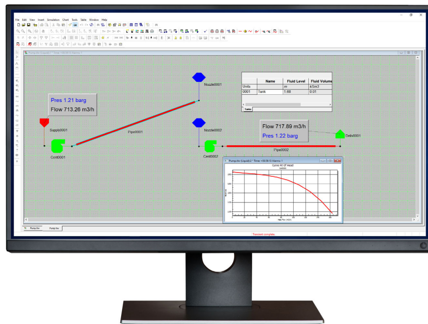
Figure 7: Gain complete visibility into flow rates, pumps, nozzles, and tanks throughout the network to enhance decision making.
